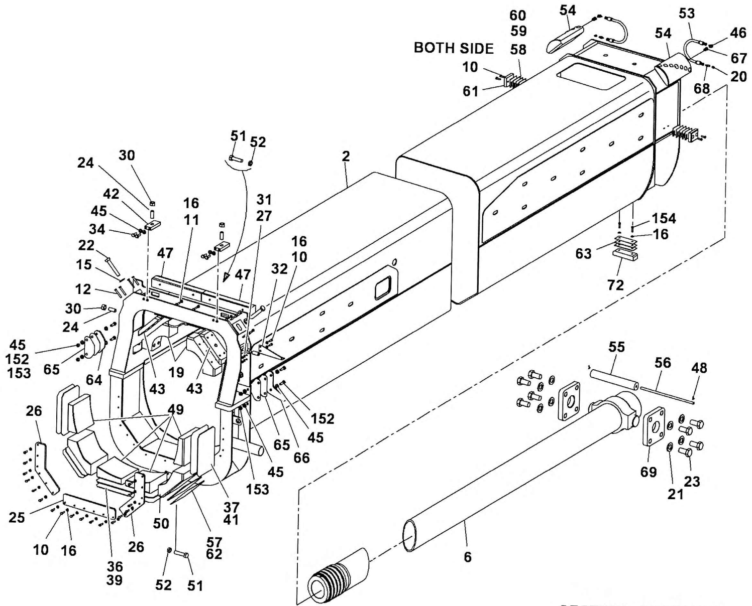
SECTION - INNER MID
